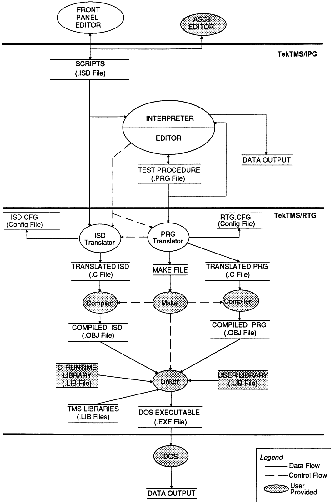
Figure 1-0 TekTMS/RTG capability.
